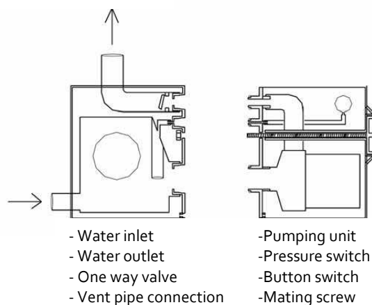
*Illustration Diagram representing the split system
