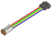
Pump adapter cable (Deutsch to Mate-n-lock)
