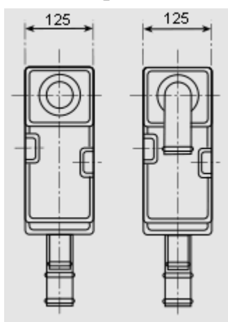
MS5005 45mm and 50mm straight outlet
