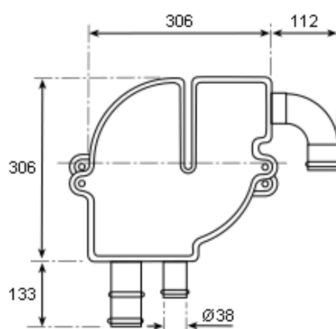
MS5020 45mm and 50mm 90 degree outlet
